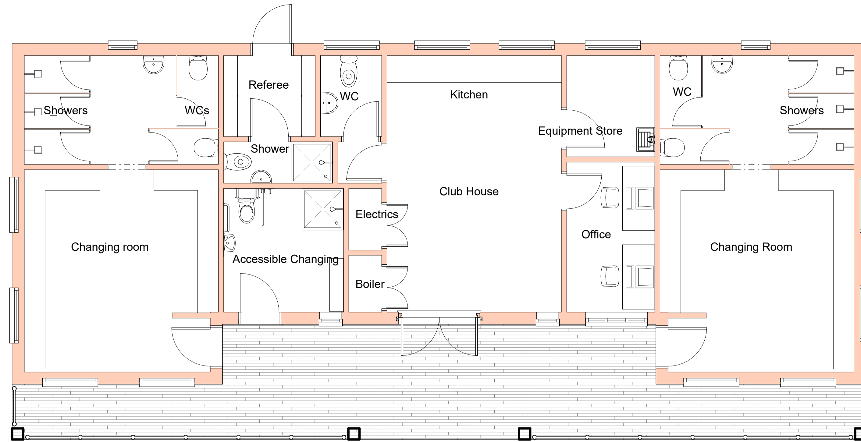
Ground Floor as proposed 1 : 50
